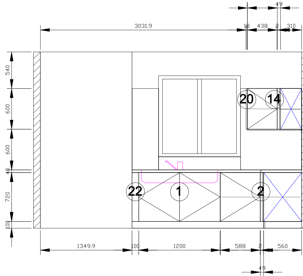
C View elevation drawing
